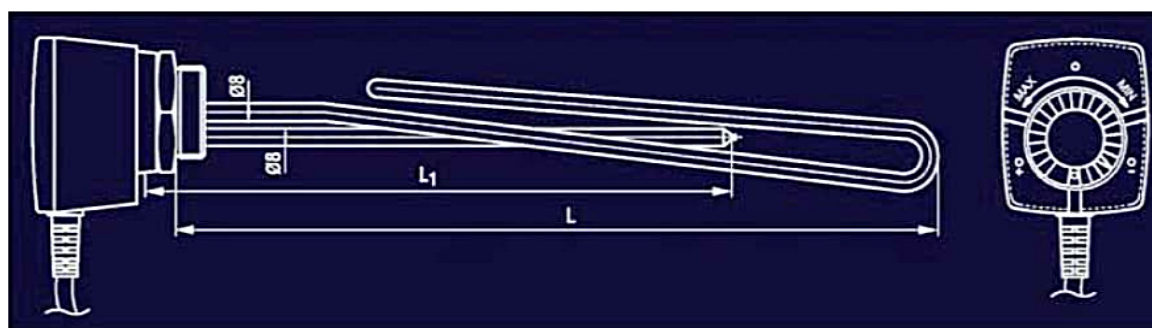
3 kW/ 230 V
